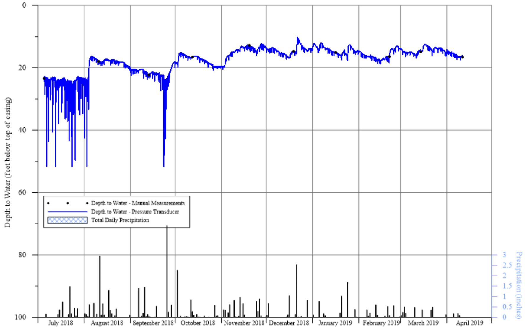
Well Monitoring Program Hydrograph of Water-Level Measurements Collected from Well C
